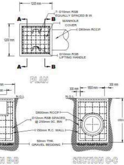
2 P 7 CATCH PIT DETAIL SCALE 1:50 M
