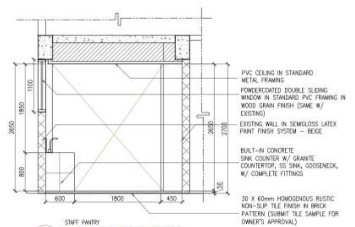
2 A-5 STAFF PANTRY CROSS SECTION SCALE: 1:50 MTS
