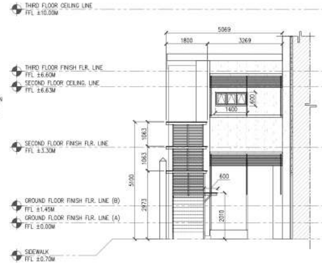
5 A-6 KITCHEN STAIRS FRONT ELEVATION SCALE 1:100 MTS
