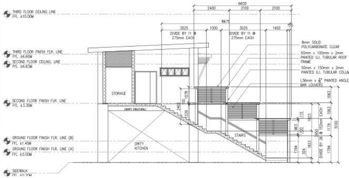
4 A-6 KITCHEN STAIRS SECTIONAL ELEVATION SCALE 1:100 MTS
