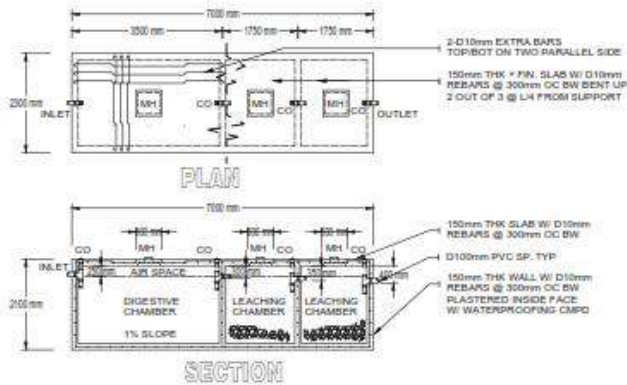
1 P 7 SEPTIC TANK DETAIL SCALE 1:100 M
