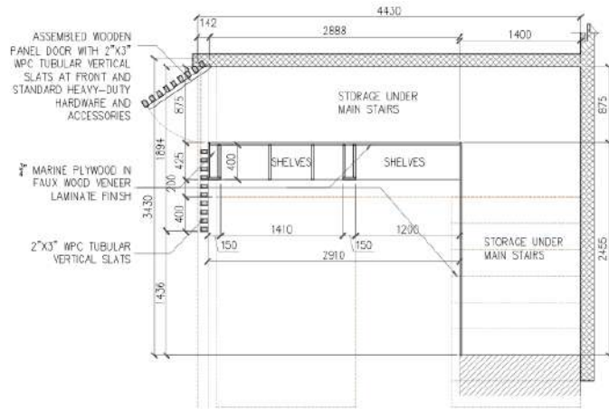
1 BLOW-UP PLAN SCALE: 1:50 MTS
