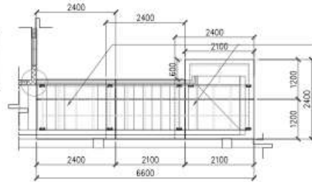
2 A-6 KITCHEN STAIRS ROOF PLAN SCALE 1:100 MTS
