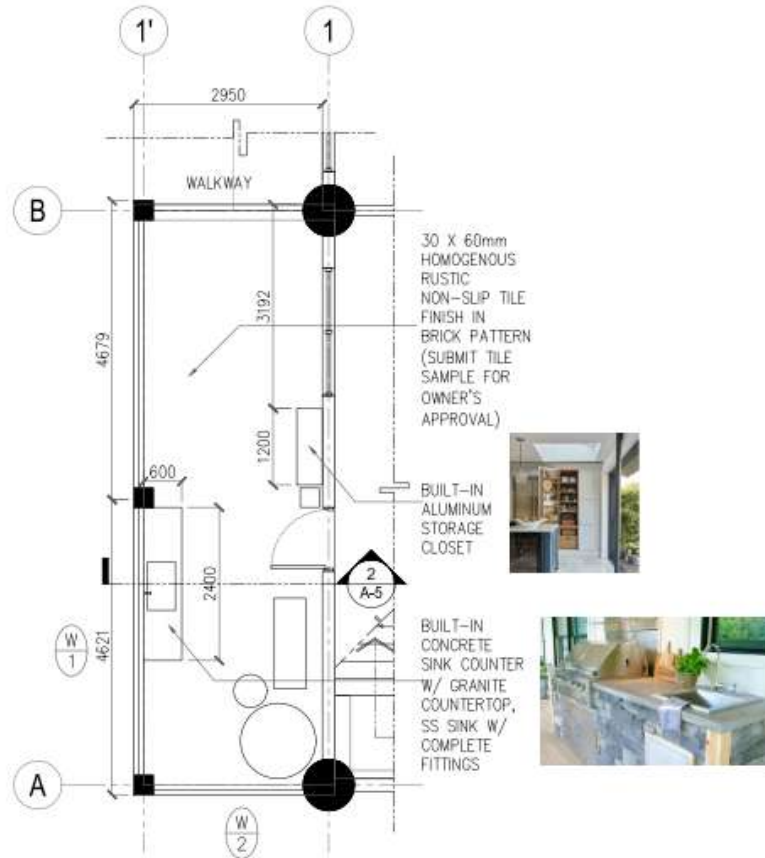
1 A-5 STAFF PANTRY FLOOR PLAN SCALE: 1:75 MTS
