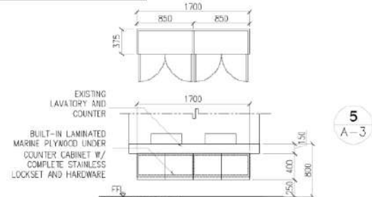
4 TYPICAL FRONT ELEVATION SCALE: A-3 1:50 MTS
