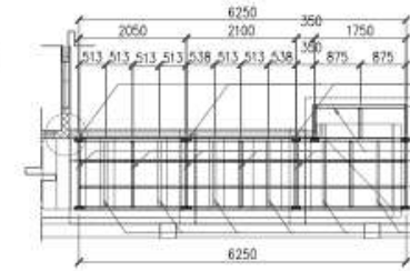
3 A-6 KITCHEN STAIRS ROOF FRAMING PLAN SCALE 1:100 MTS
