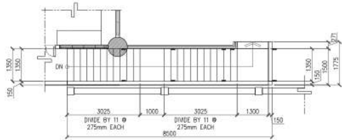
1 A-6 KITCHEN STAIRS FLOOR PLAN SCALE 1:100 MTS
