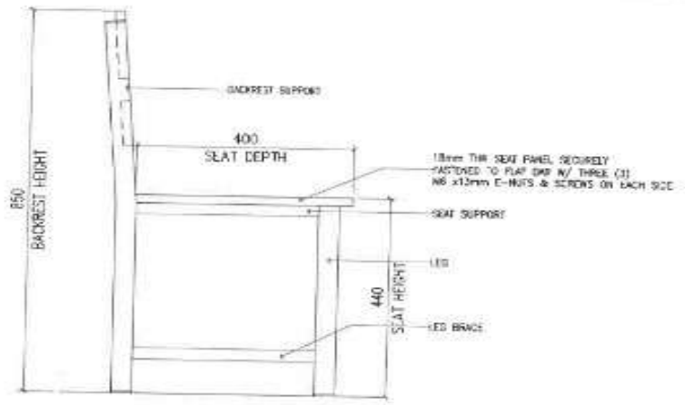
3 LEFT-SIDE ELEVATION SCALE 1:100 M
