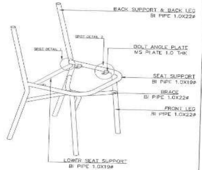
PERSPECTIVE VIEW
