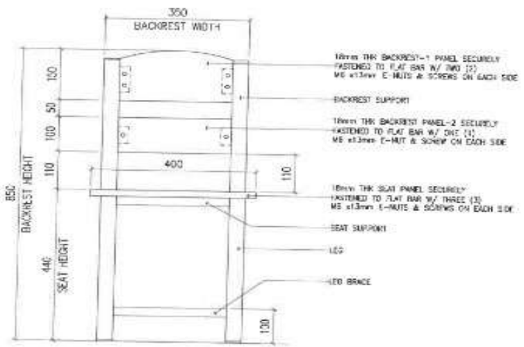
2 FRONT ELEVATION SCALE 1:100 M
