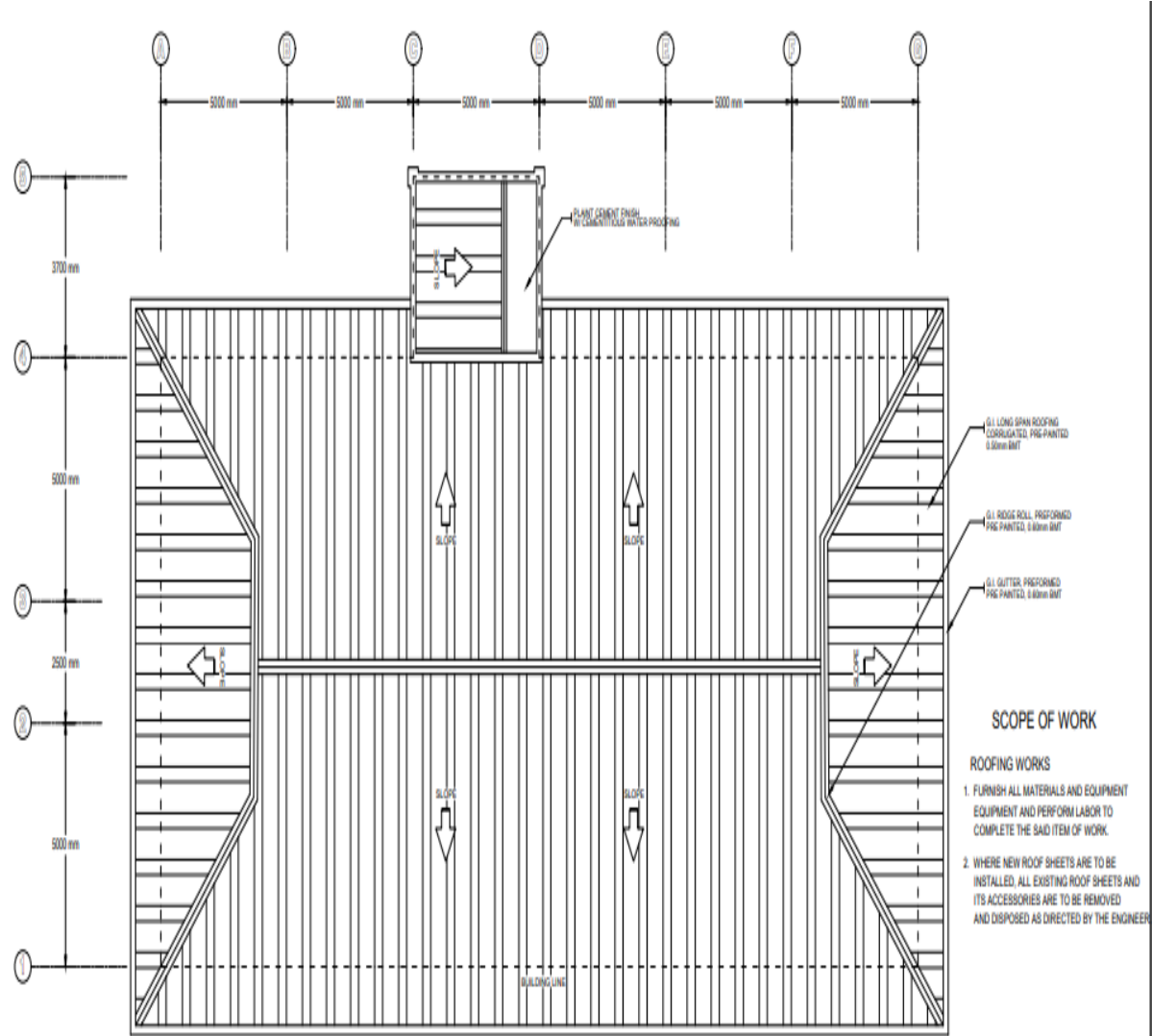
1 ROOF PLAN SCALE 1:100M
