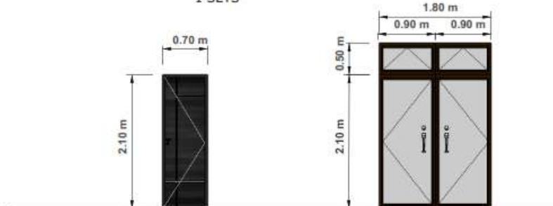
D 1 ANALOC ALUMINUM SWING DOOR WITH AWNING WINDOW WITH 1/4" THK CLEAR CLASS 1 SET
