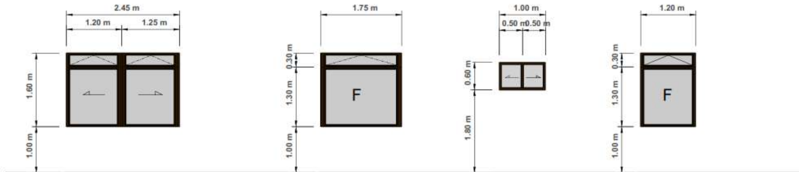
W 2 ANALOC ALUMINUM AWNING AND FIXED WINDOW WITH 1/4" THK CLEAR CLASS 1 SETS
