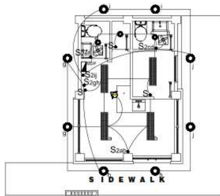
GUARD HOUSE LIGHTING LAYOUT SCALE: 1:100 M
