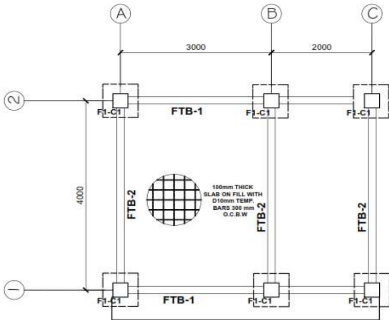
1 FOUNDATION PLAN DRAWN NOT TO SCALE
