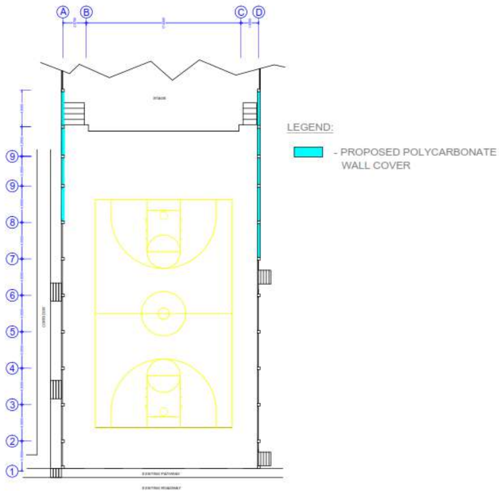
1 LOCATION OF POLYCARBONATE WALL COVER Scale: 1:100
